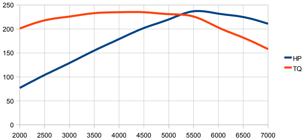
Stock 3500 with Strip Cam
