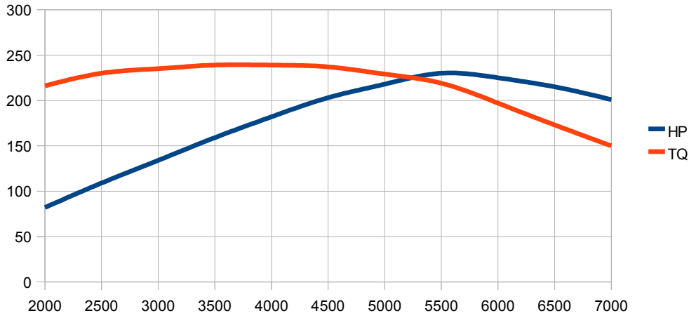
Stock 3500 with Street/Strip Cam
