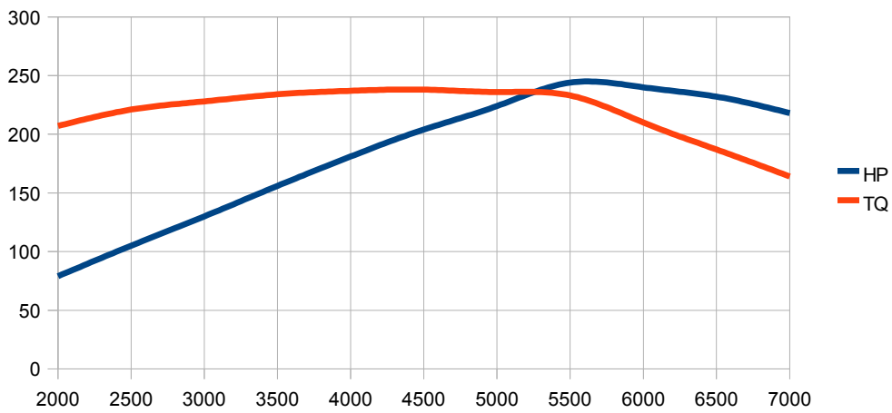
Stock 3500 with Race Cam
